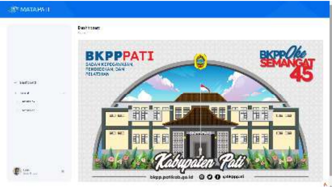
Gambar 2. Halaman Dashboard
